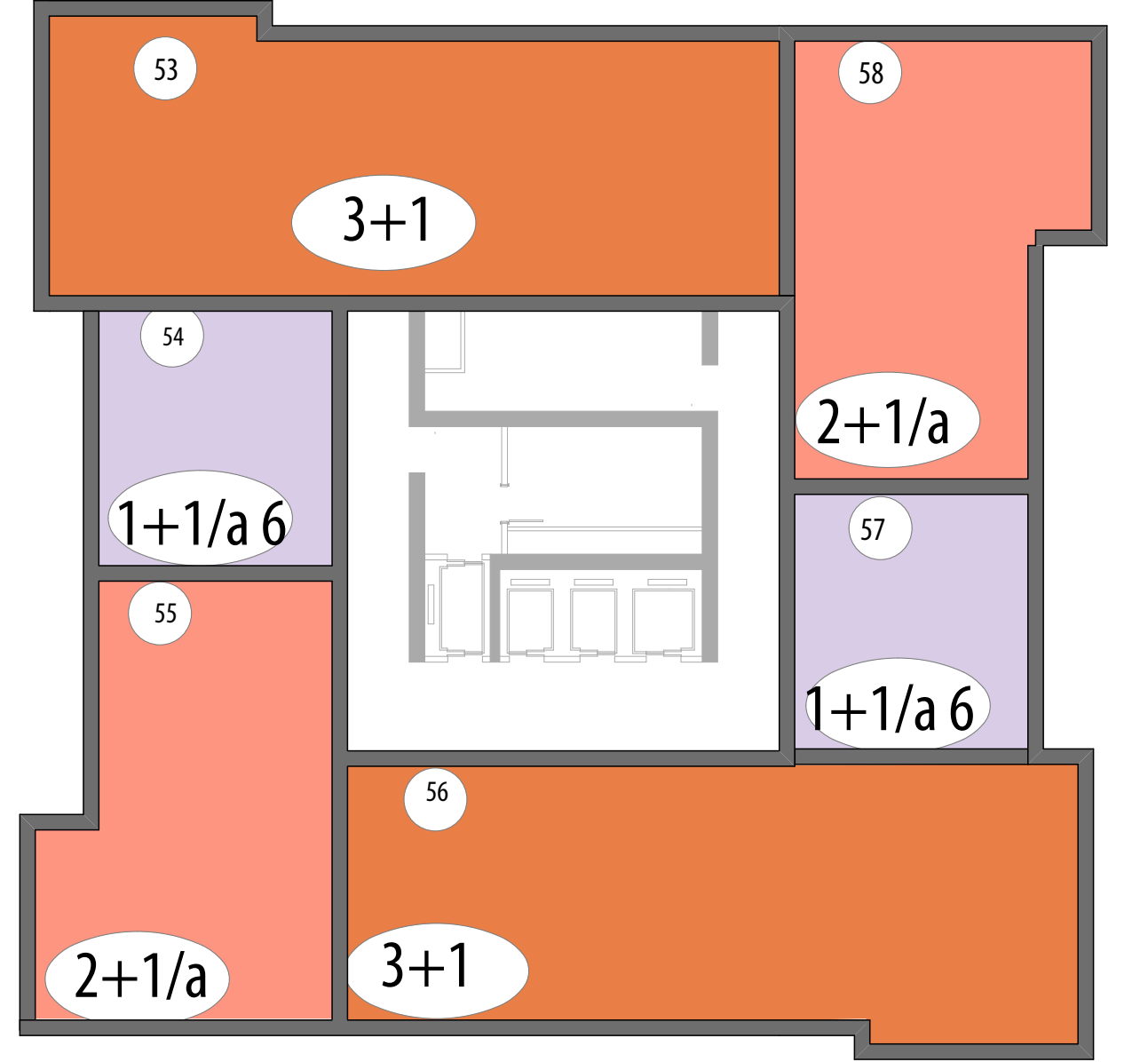
B-C-E-F BLOK 8. KAT PLANI
